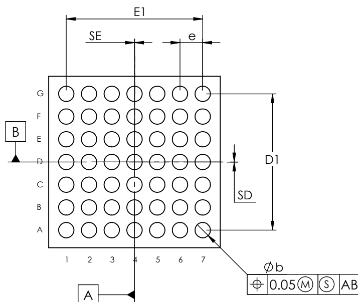
BOTTOM VIEW
