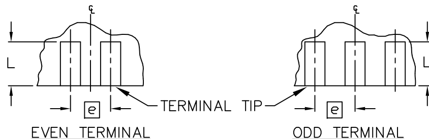
DETAIL 'A'
