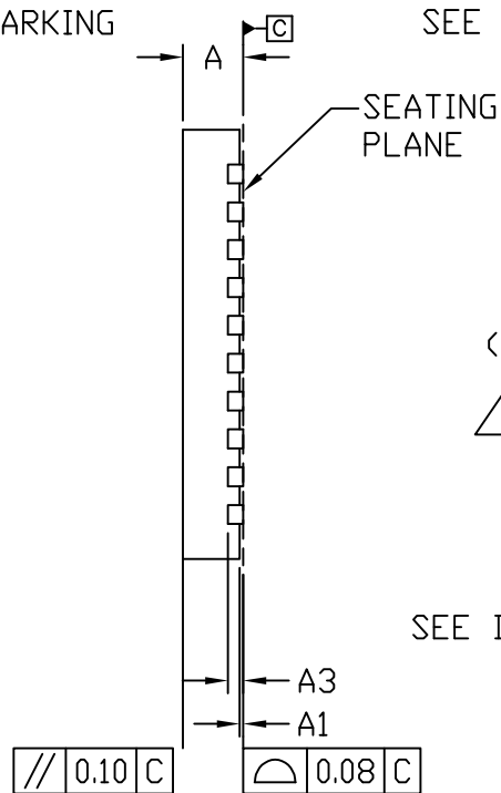
SIDE VIEW
